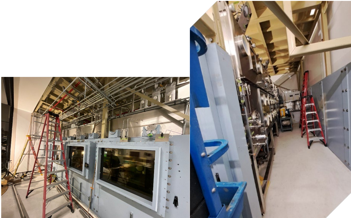
Figure 16 Photographs of MSTEC shield walls and glove box undergoing installation in FCF.
