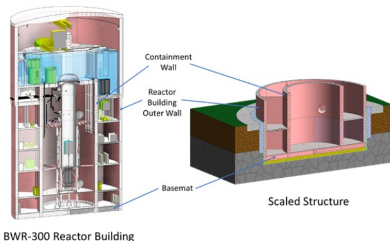
Figure 7 BWRX-300 reactor building and ACTI scaled structure
