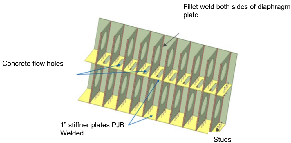
Figure 9 DPSC diagram
