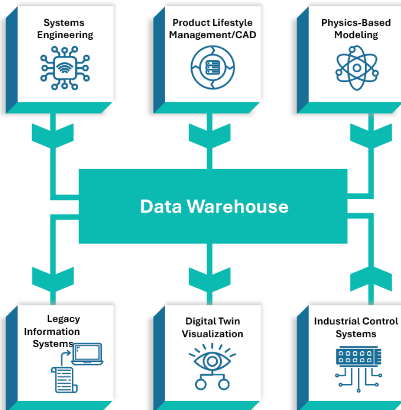
Figure 12 Data warehouse
