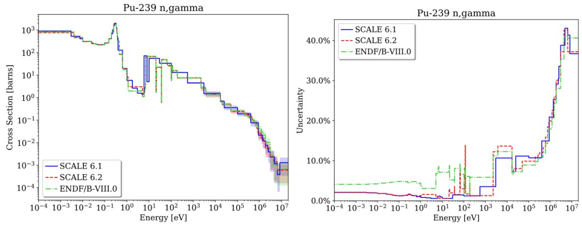
Figure 46. ^{239}\text{Pu} (n,γ) cross section and uncertainty.
