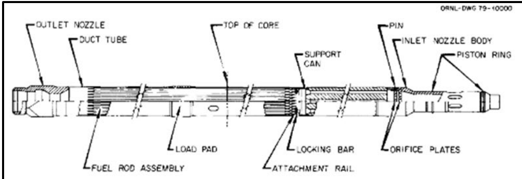
Fig. 4. LMFBR fuel assembly.
