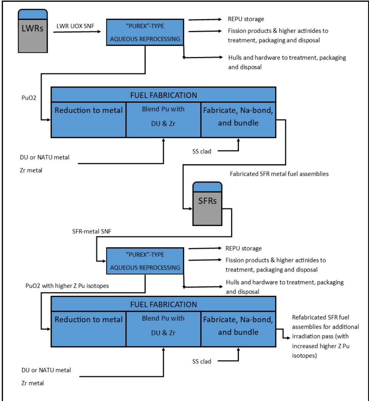
Figure D1-6B.3 shows how this first SFR pass spent fuel can be reprocessed in order to provide refabricated U,Pu metal fuel for second-pass SFR use. Additional SFR-passes are possible with aqueous SFR fuel reprocessing capacity; however, each pass results in (1) recovered Pu with higher content of undesirable Pu higher isotopes and (2) the need to bump up the refabricated fuel’s fissile content above the 15 to 20% fissile content typical of CRBRP-type SFRs operated in a breeding or high conversion mode. The refabricated SFR-SNF-derived U,Pu-metal FMF will likely require some more stringent design and operational requirements as a result of its higher radioactivity and heat generation during handling. Thicker glovebox windows and remote (robotic) maintenance of the fabrication line may be required to keep the facility remaining as a contact-handling class plant operating under ALARA (as low as reasonably achievable) personnel protection regulations. As will
